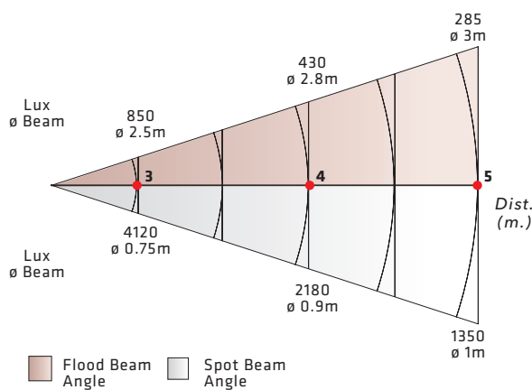
FRESNEL LED 90W - MODEL 53-19/A
